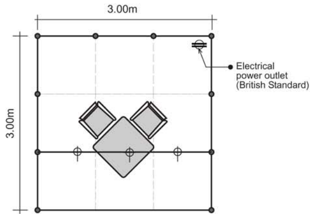
Floor Plan
